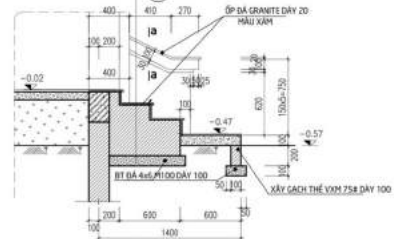
CẮT 10-10 (T.L: 1/25)
