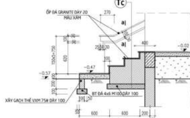
CẮT 11-11 (T.L: 1/25)
